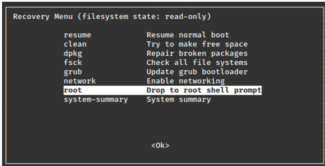
Fig. 4: Recovery Menu
